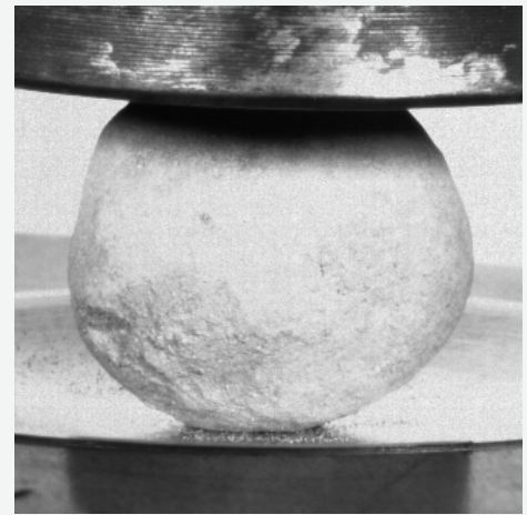
Sponge iron pellets reduced with hydrogen have a high degree of metallisation (98-99%) and 0% carbon. Measurements show that they have higher compressive strength than pellets produced with natural gas.
